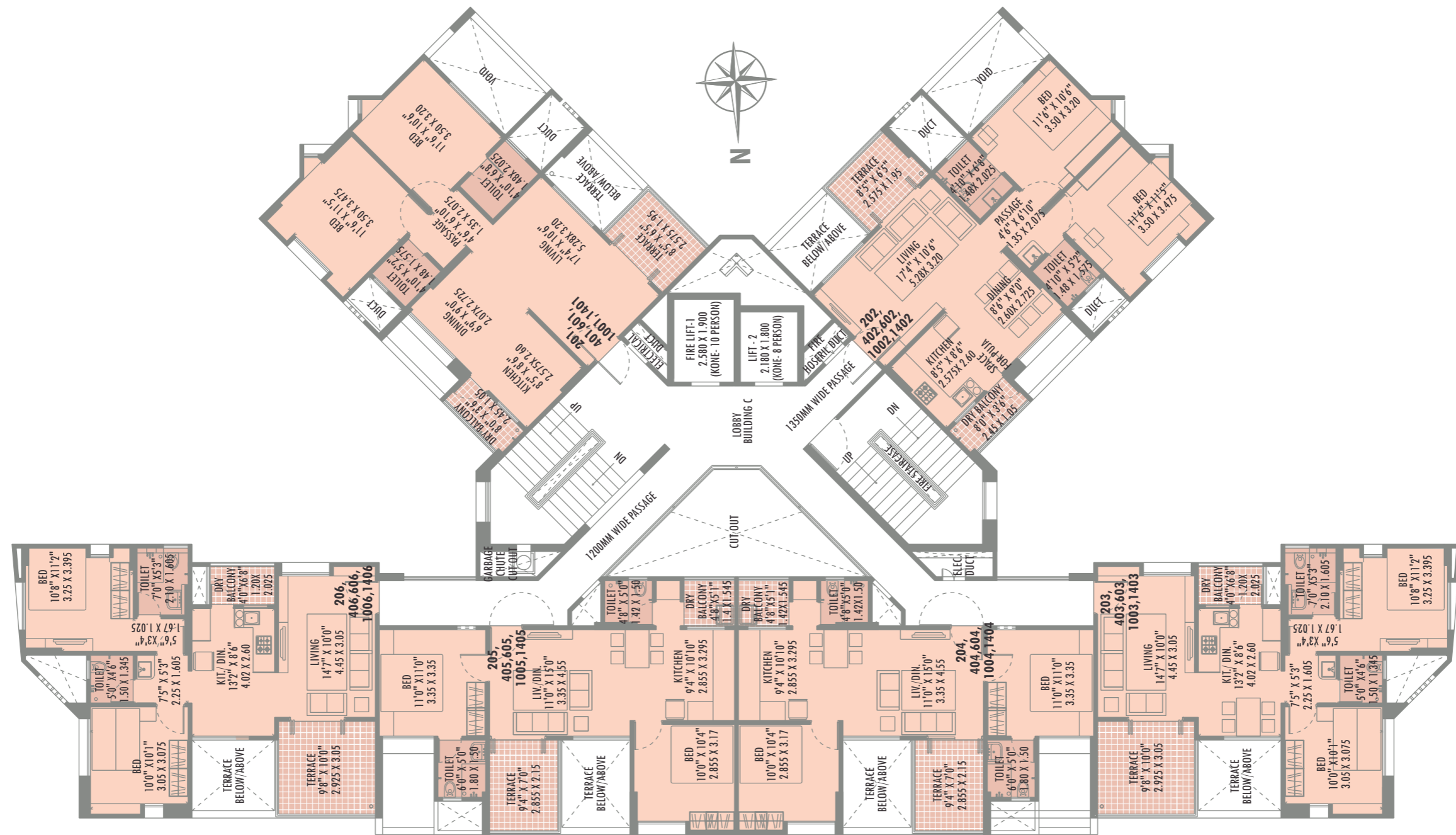
TYPICAL 2ND, 4TH, 6TH, 10TH & 14TH FLOOR
